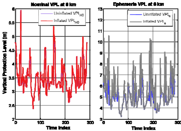
Figure 3: VPL Inflation Required to Remove Unsafe Geometries
