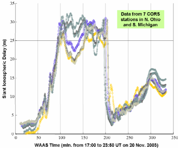
Figure 1: Ionospheric Delay on SVN 38 During 20/11/2003 Anomaly
